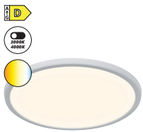
Oja 29 2210656101 White | Plastic | LED Module 17W 1700lm | 3000/4000K H: 2,3 cm | Ø: 29,4 cm
