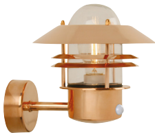
Blokhus Up Sensor 25031030 Copper | Copper Excl. E27 | Max. 60W H: 23 cm | Ø: 22 cm
