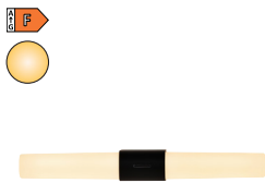
Helva 2015311003 Black | Plastic LED Module 9W | 900lm | 3000K W: 5,7 cm | L: 42,5 cm
